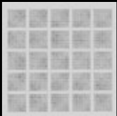
AL-013 Open area: 7.1% Weight: 0.717kg Size: 600mm x 600mm
