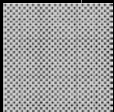
AL-046 Open area: 26.8% Weight: 0.580kg Size: 600mm x 600mm
