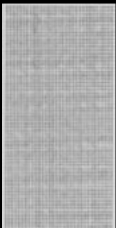
AL-056 Open area: 27.3% Weight: 1.061kg Size: 600mm x 1200mm
